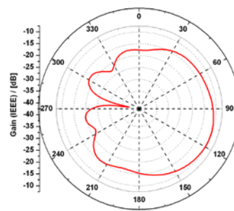
Omnidirectional antenna, vertical view
