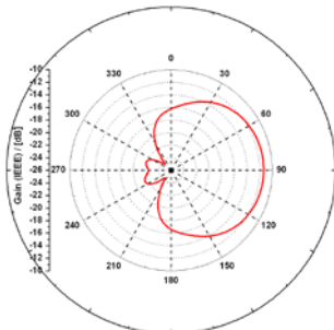
Omnidirectional antenna; horizontal view
