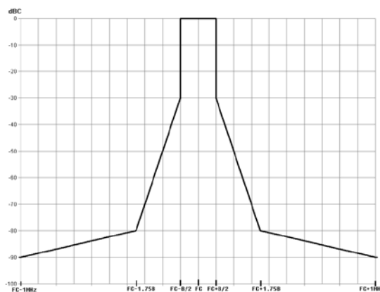
Figure A5.7: Emission mask – for digital modulation below 1 GHz; B ≤ 200 kHz
