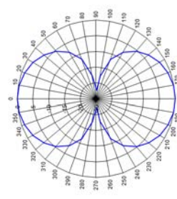
Omnidirectional antenna, vertical view
